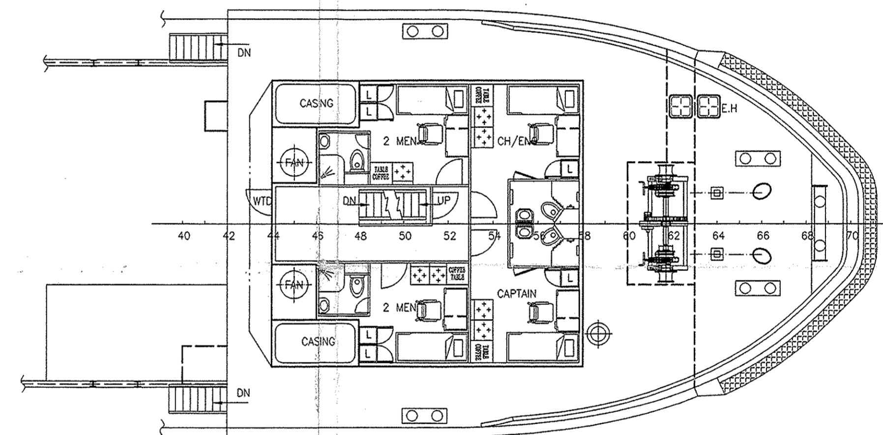
FORECASTLE DECK
