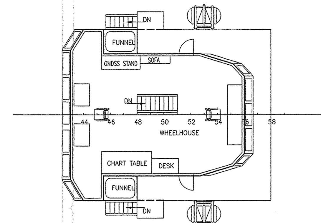
WHEELHOUSE DECK PLAN
