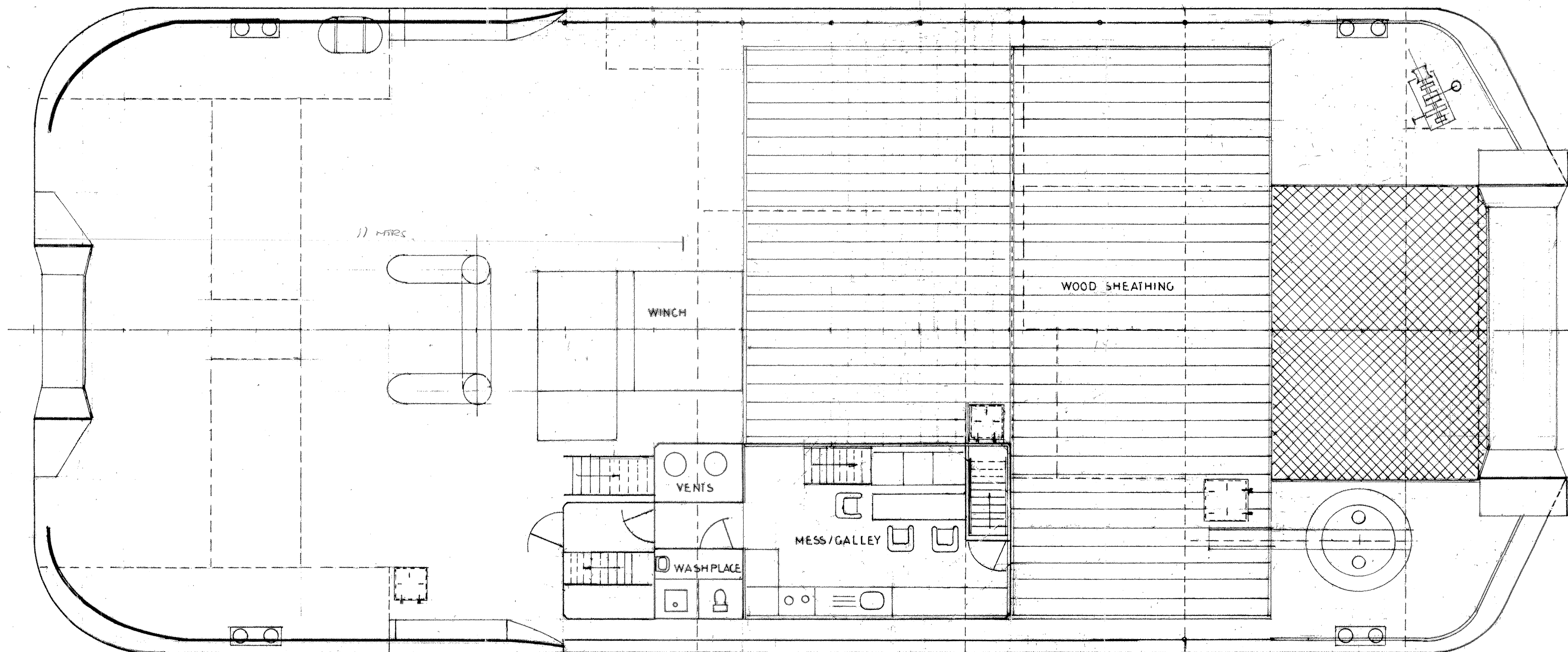
DECK PLAN
