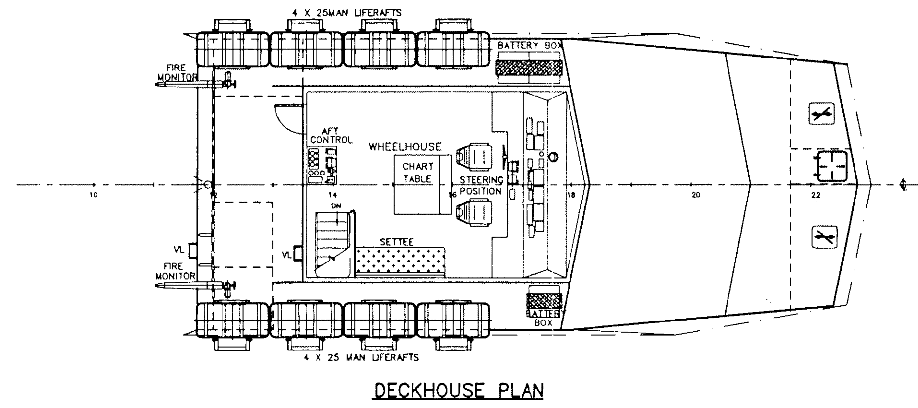
DECKHOUSE PLAN
