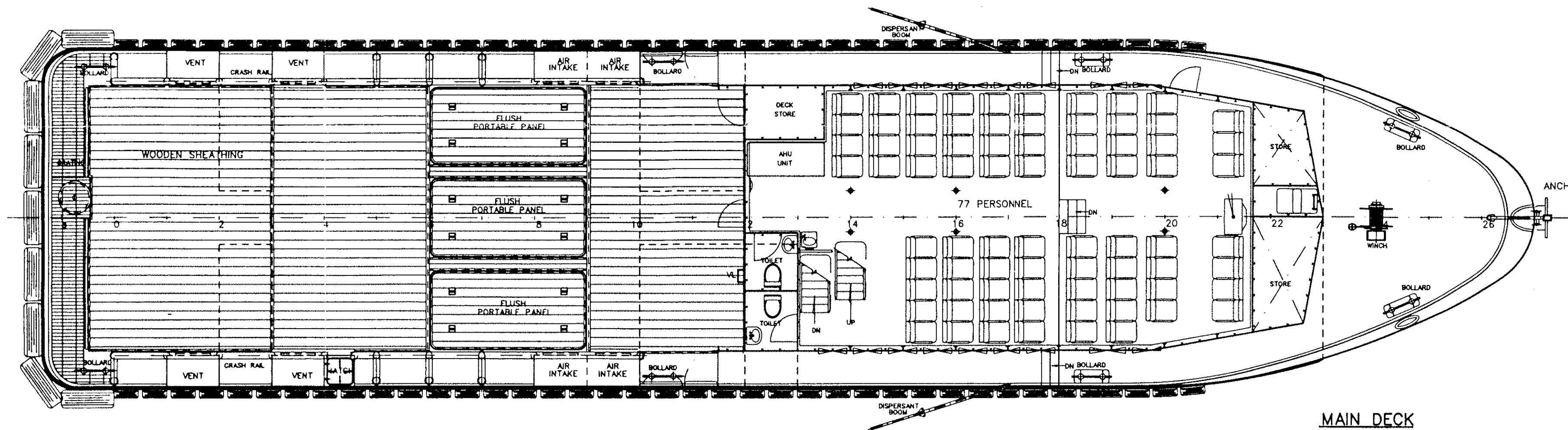
MAIN DECK
