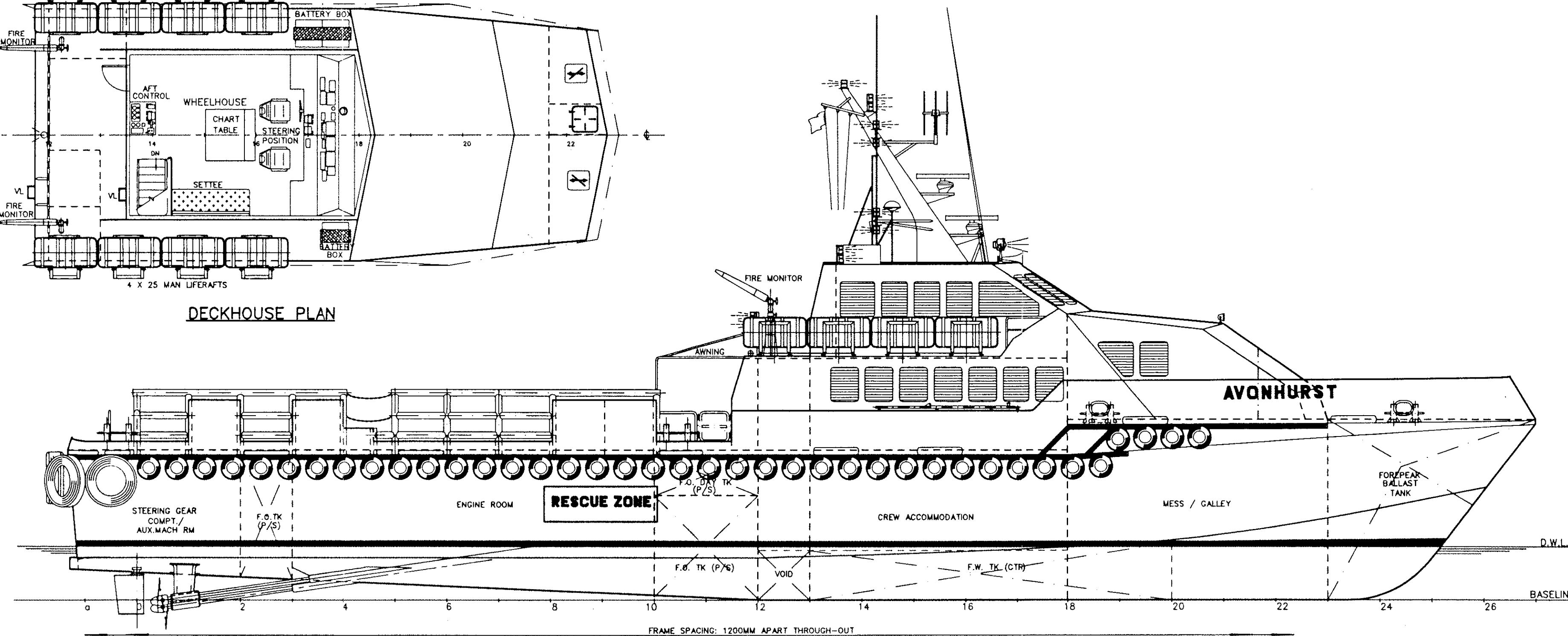
PROFILE
