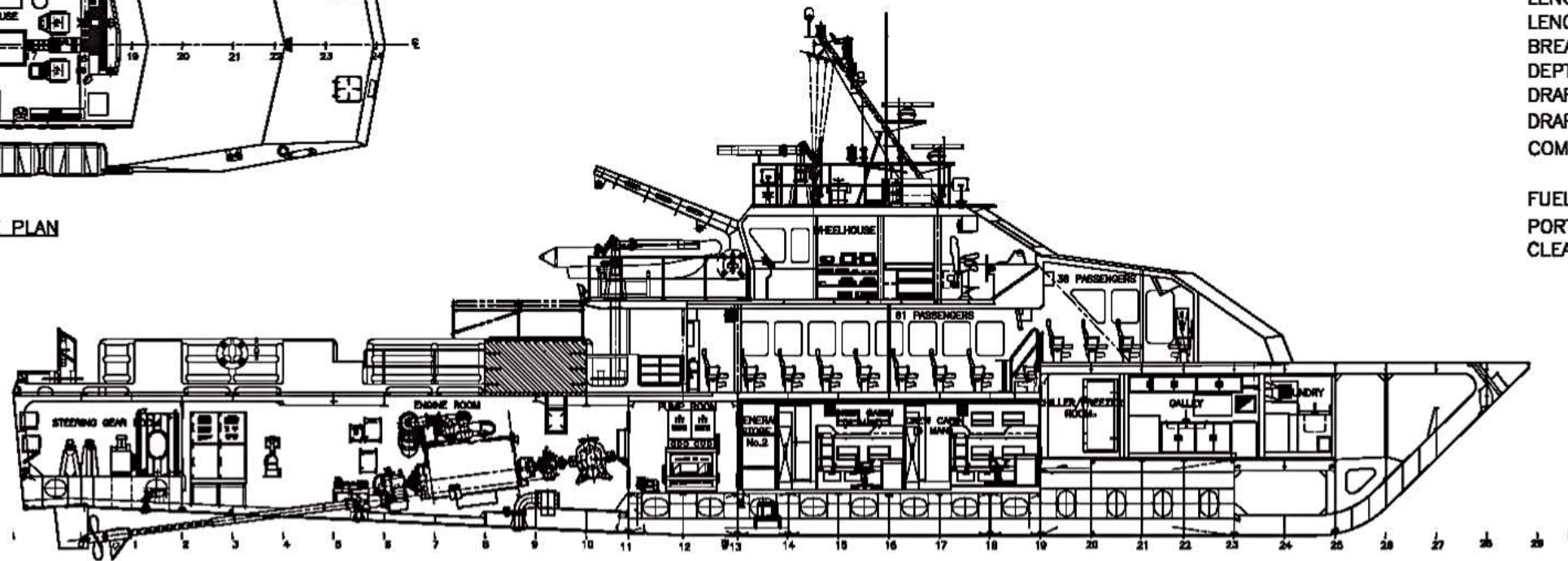
PROFILE SCALE 1/75
