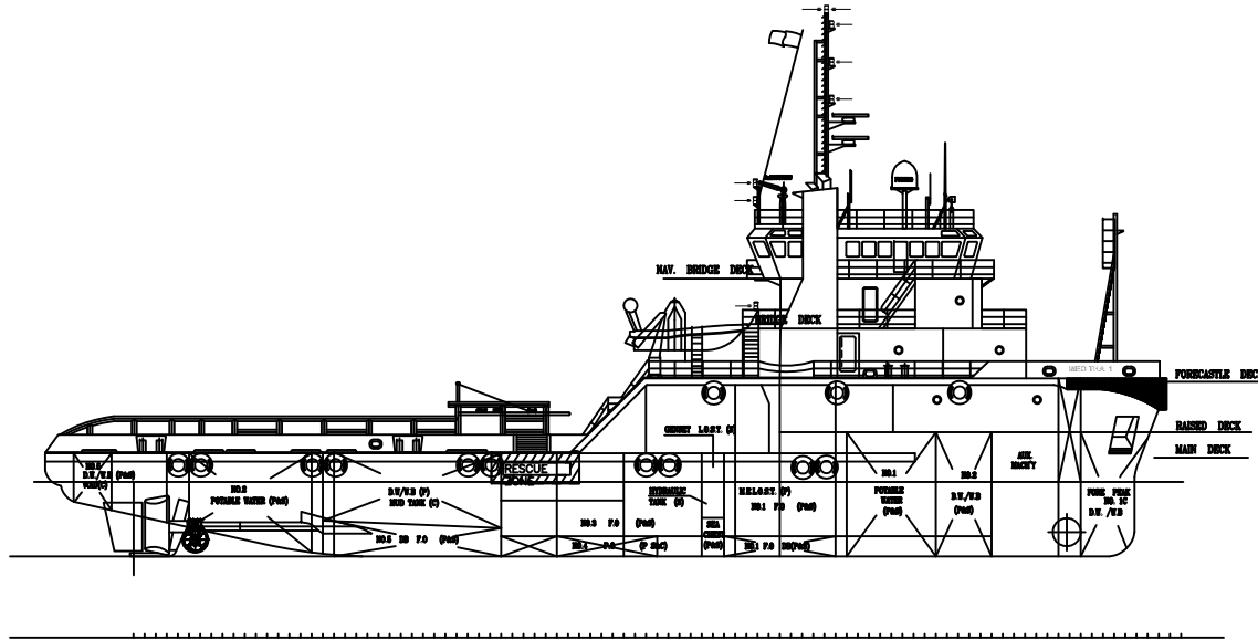
OUTBOARD PROFILE
