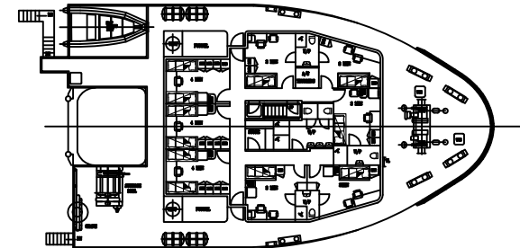
FORECASTLE DECK
