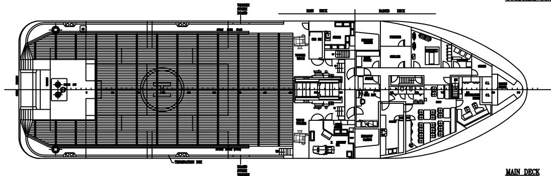
MAIN DECK
