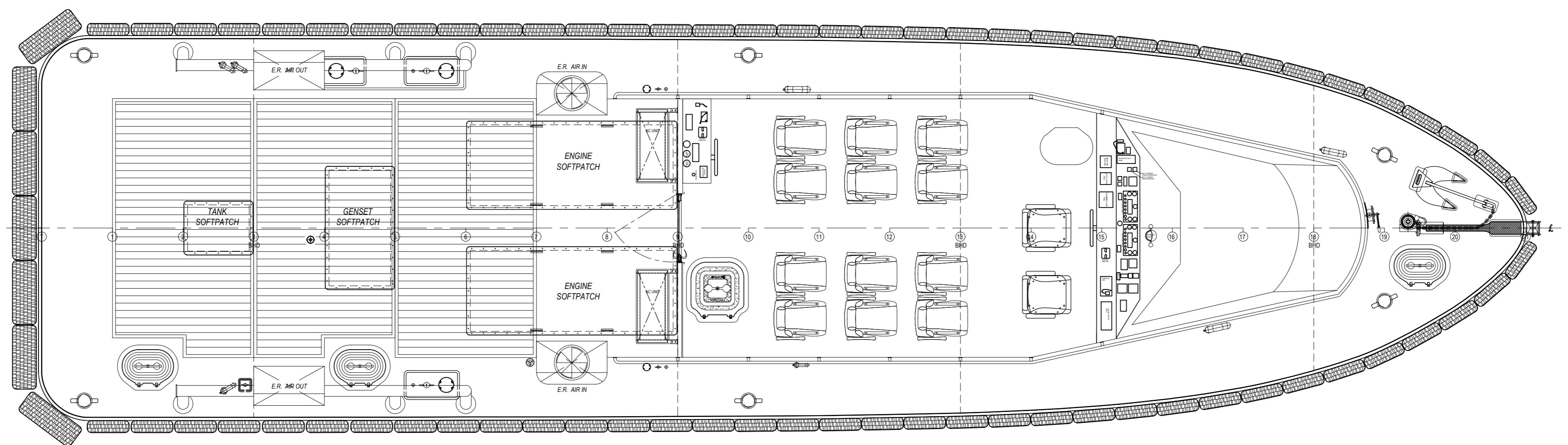
MAIN DECK PLAN
