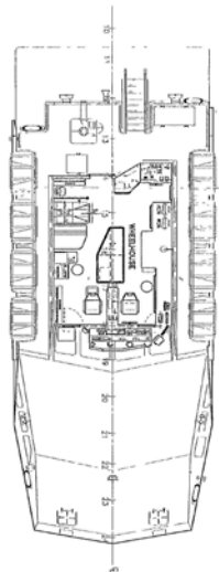
DECKHOUSE PLAN SCALE 1:75
