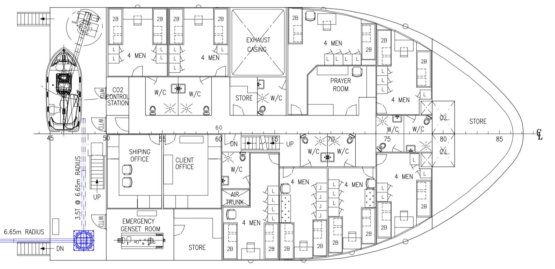
LOWER F'CSLE DECK
