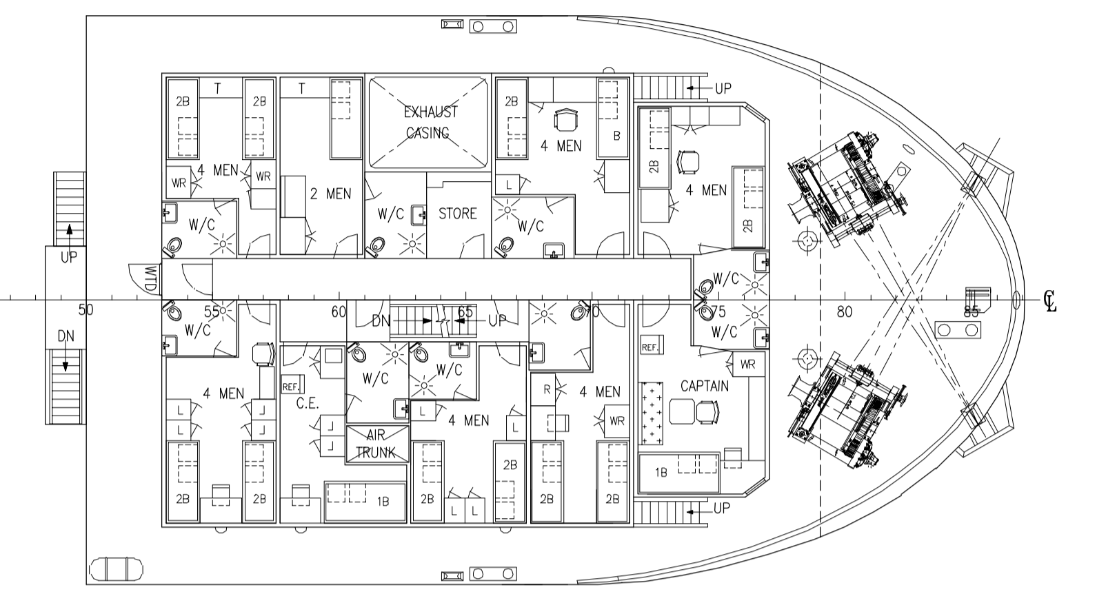
UPPER F'CSLE DECK
