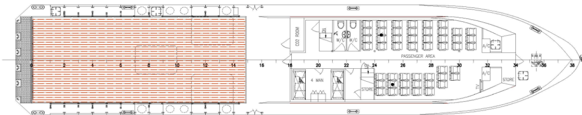
MAIN DECK
