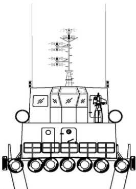
STERN VIEW
