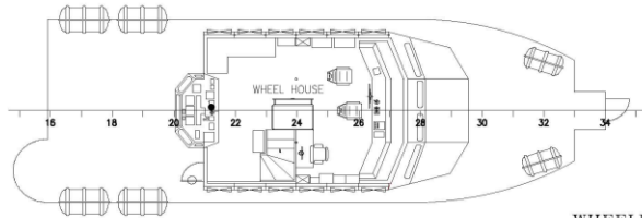
WHEELHOUSE
