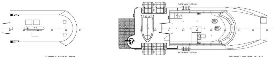
WHEELHOUSE TOP
