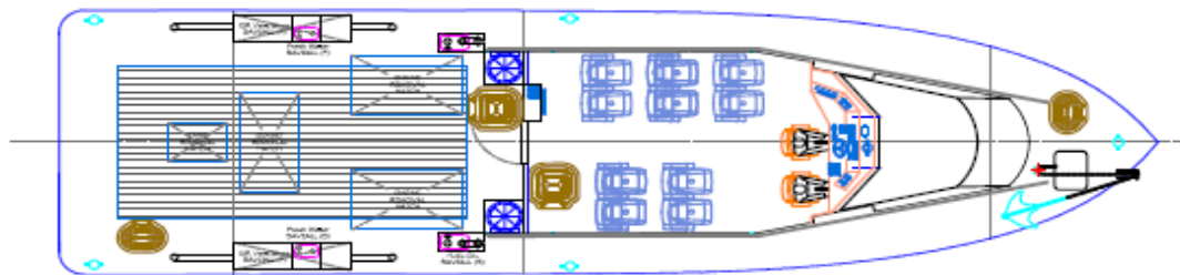
Main Deck Arrangement
