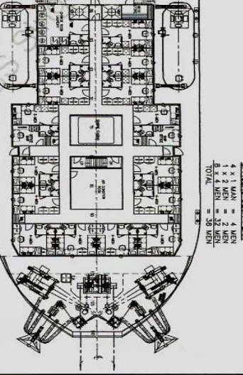
FORECASTLE DECK PLAN
