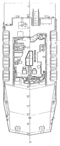
DECKHOUSE PLAN SCALE 1:10
