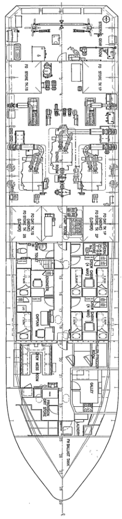
BELOW MAIN DECK SCALE 1:75
