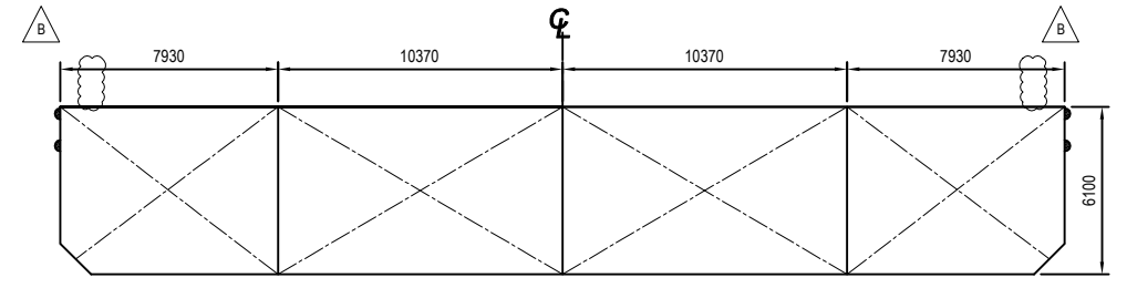
MIDSHIP SECTION
