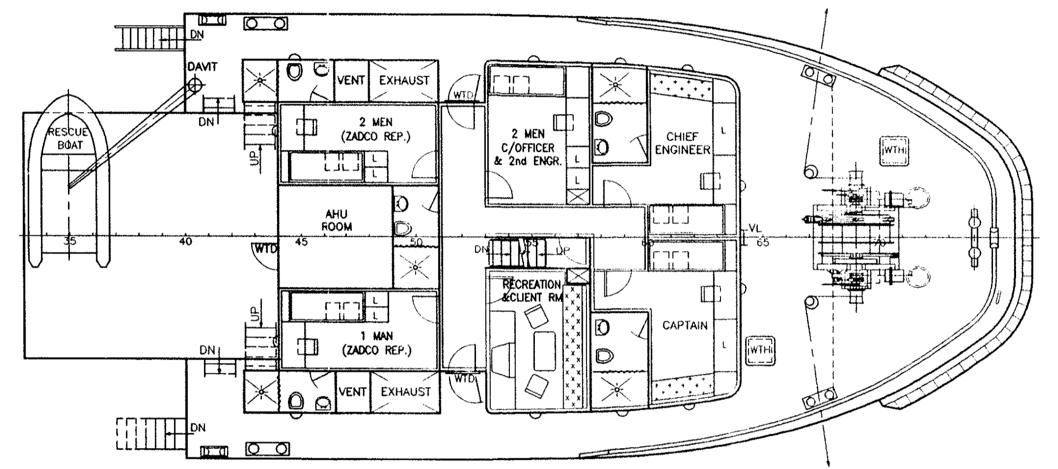
FORECASTLE DECK
