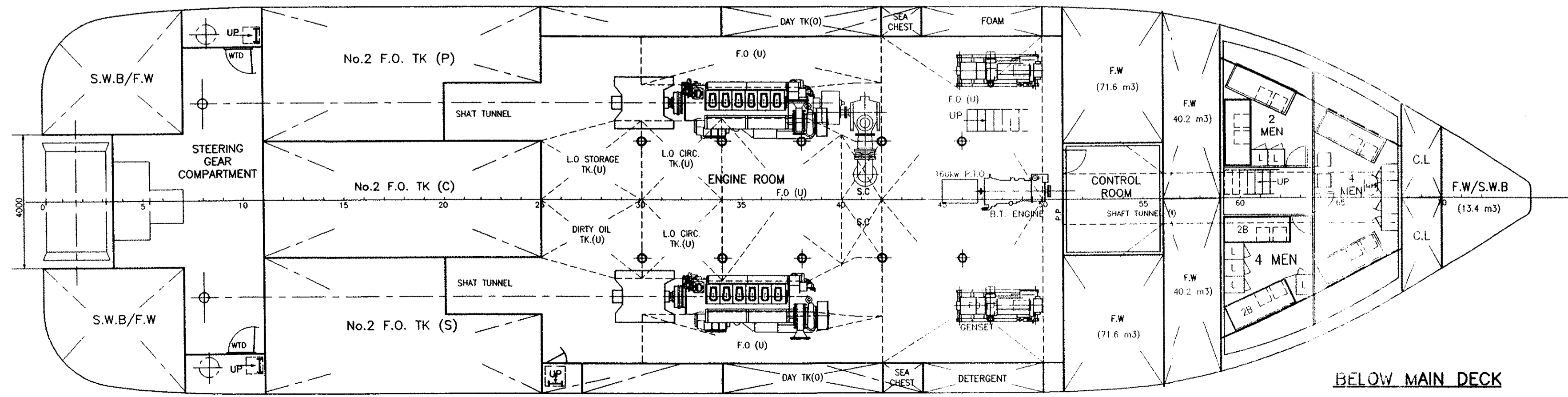
MAIN DECK
