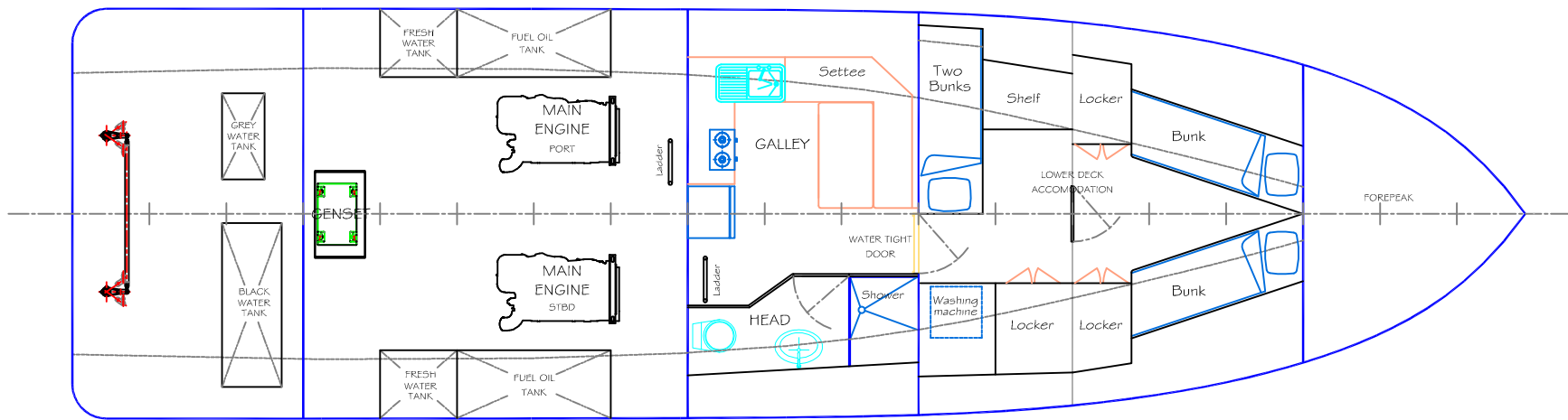
Below Deck Arrangement
