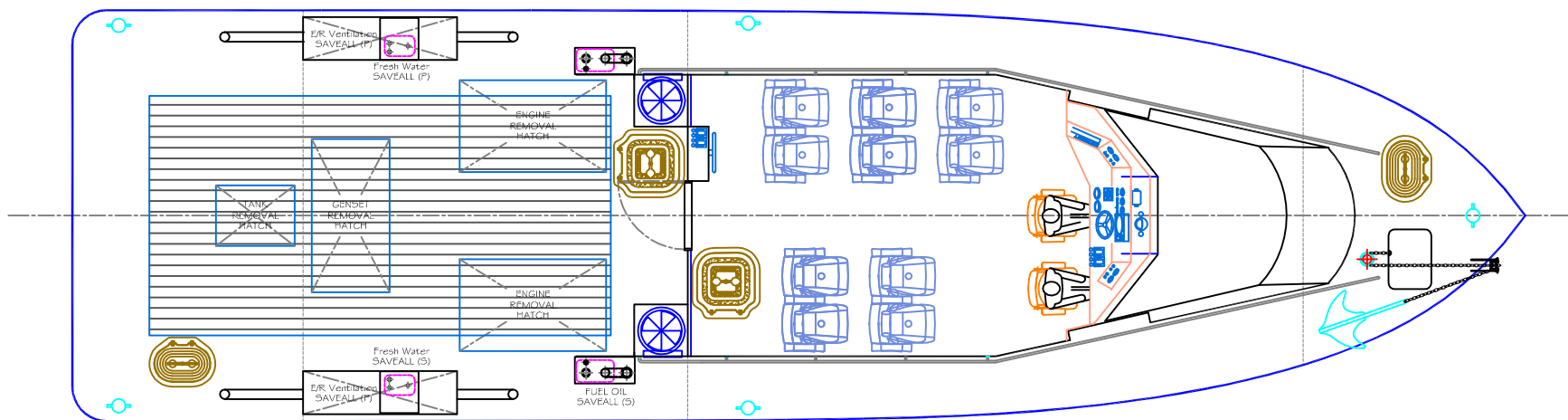
Main Deck Arrangement
