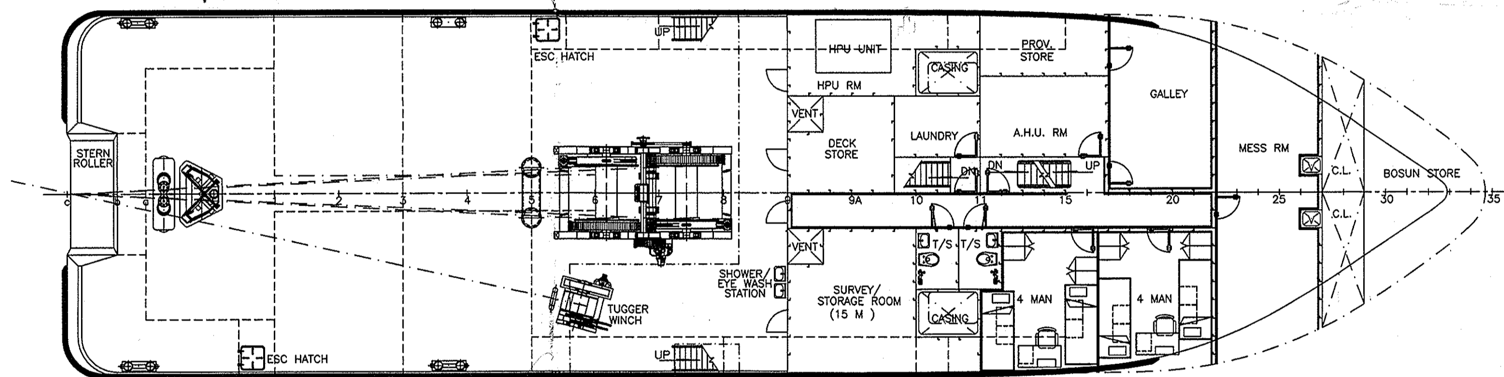
MAIN DECK PLAN
