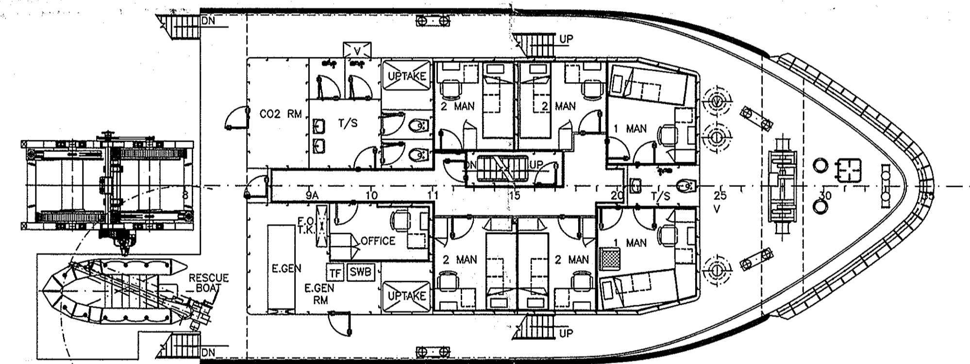
FORECASTLE DECK
