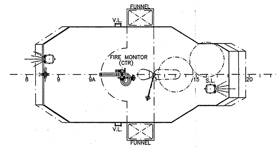
FLYBRIDGE DECK
