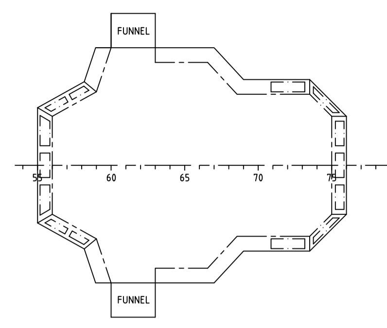
WHEELHOUSE TOP
