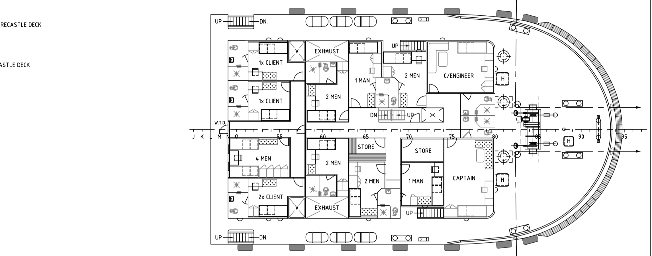
UPPER FORECASTLE DECK
