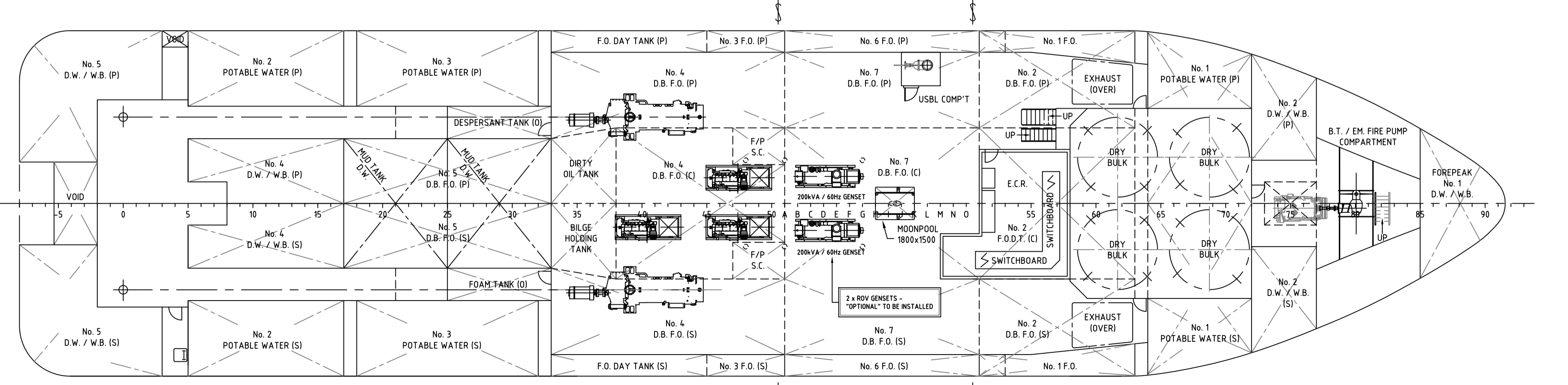
BELOW MAIN DECK
