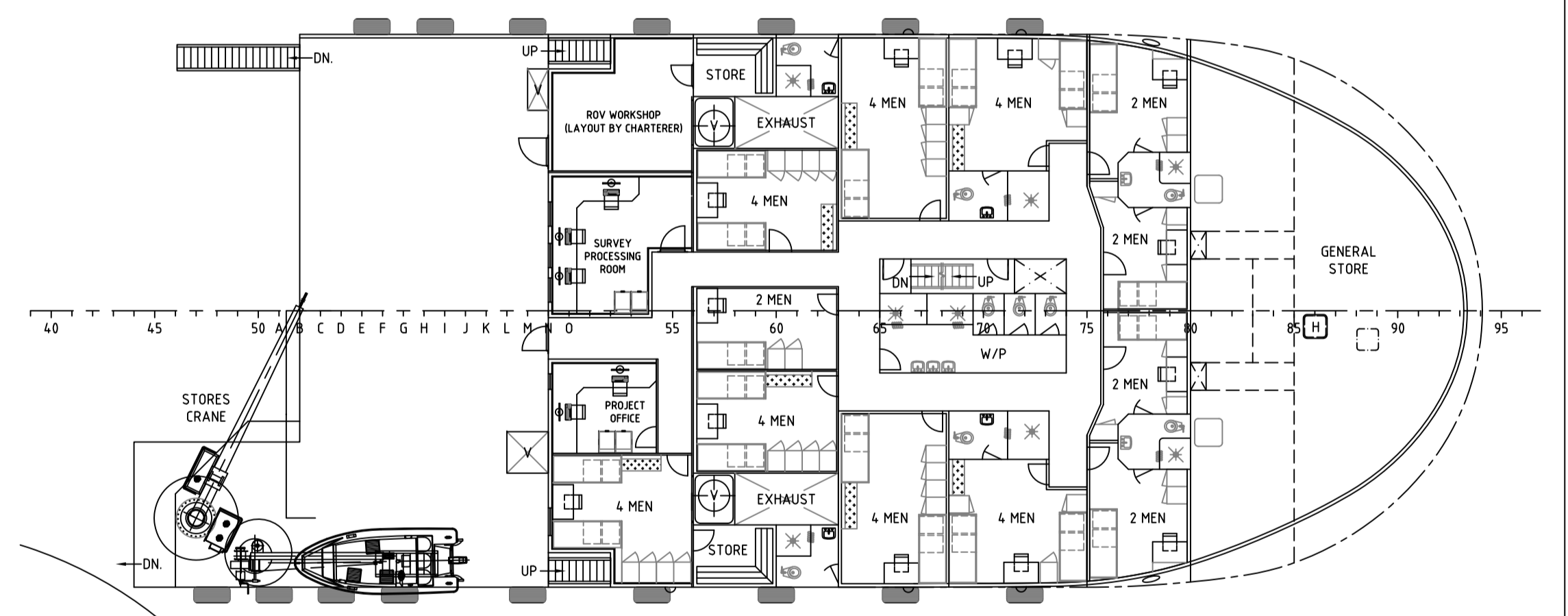
LOWER FORECASTLE DECK
