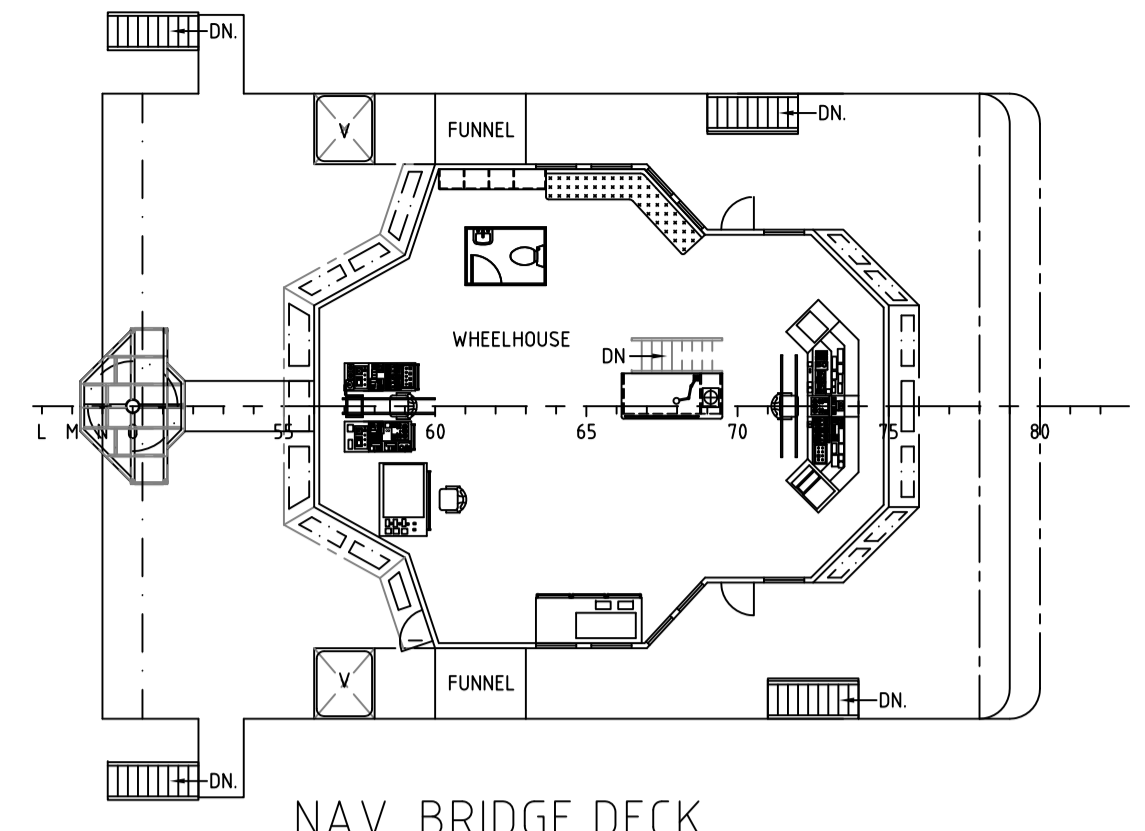
NAV. BRIDGE DECK
