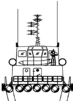
STERN VIEW
