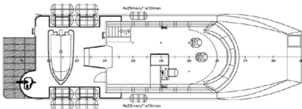
WHEELHOUSE PLAN
