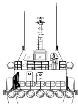
STERN VIEW
