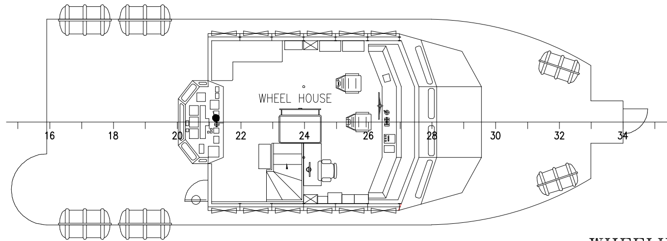
WHEELHOUSE
