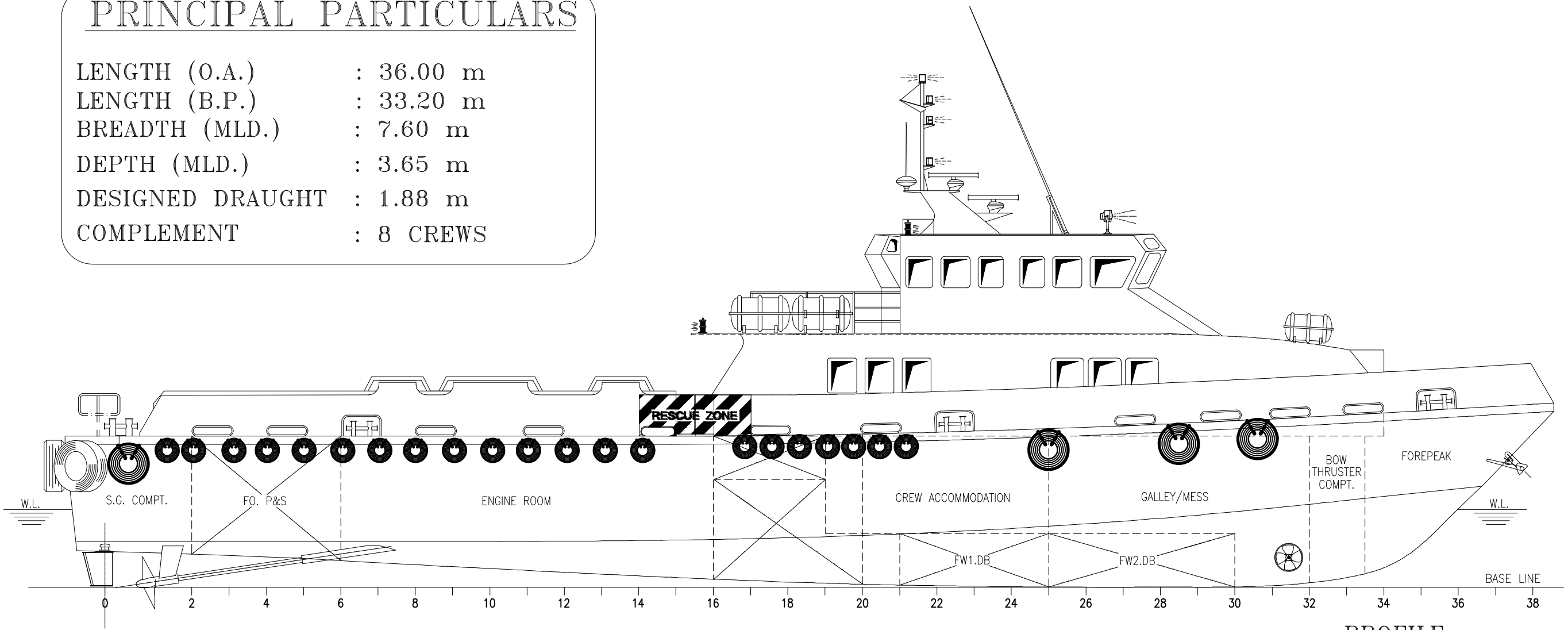
PROFILE
