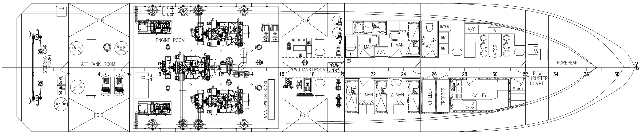
BELOW MAIN DECK
