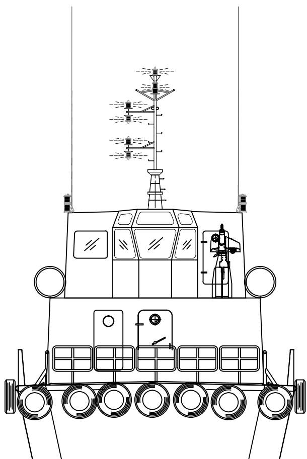
STERN VIEW
