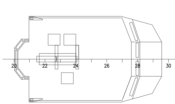
WHEELHOUSE TOP
