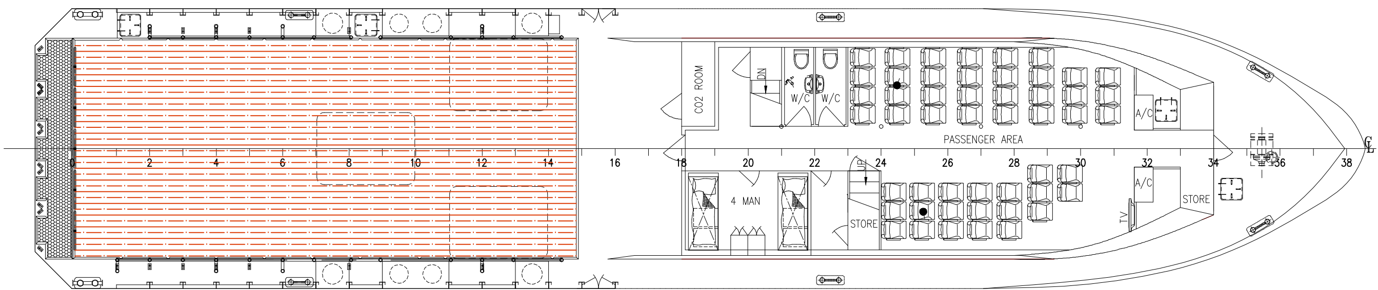
MAIN DECK
