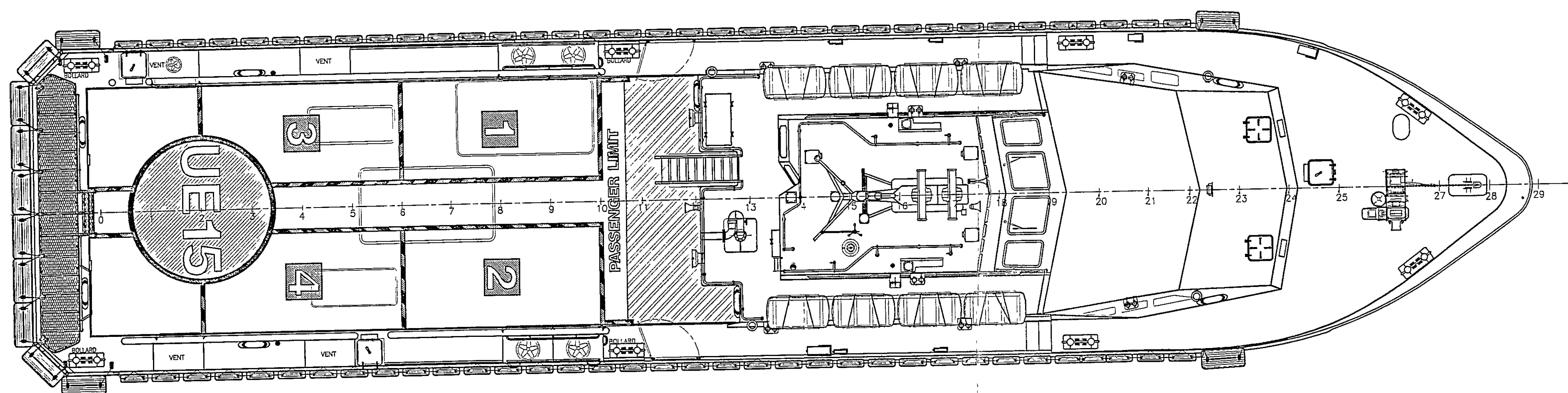
DECK PLAN SCALE 1/75
