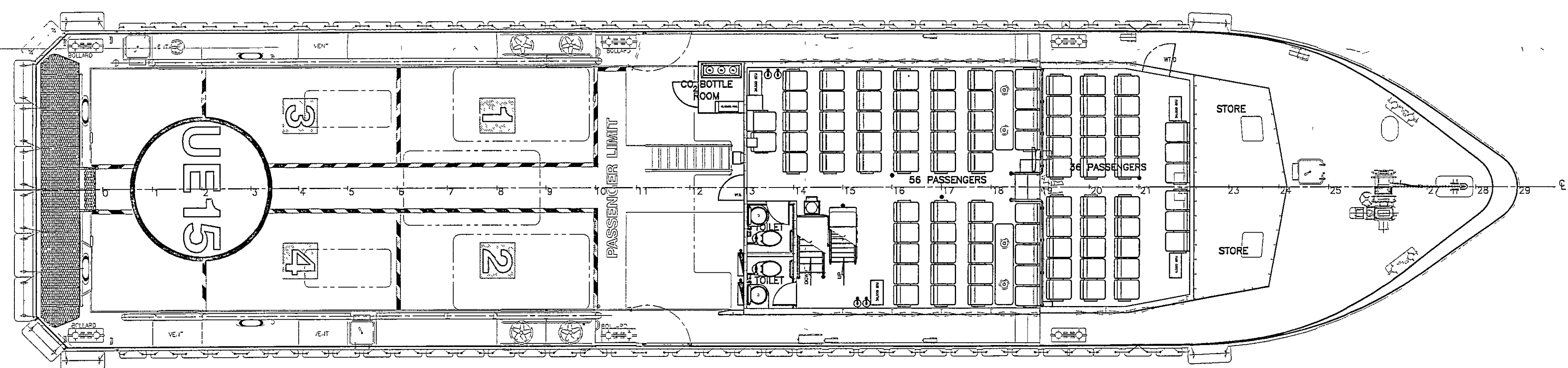
MAIN DECK SCALE 1:75
