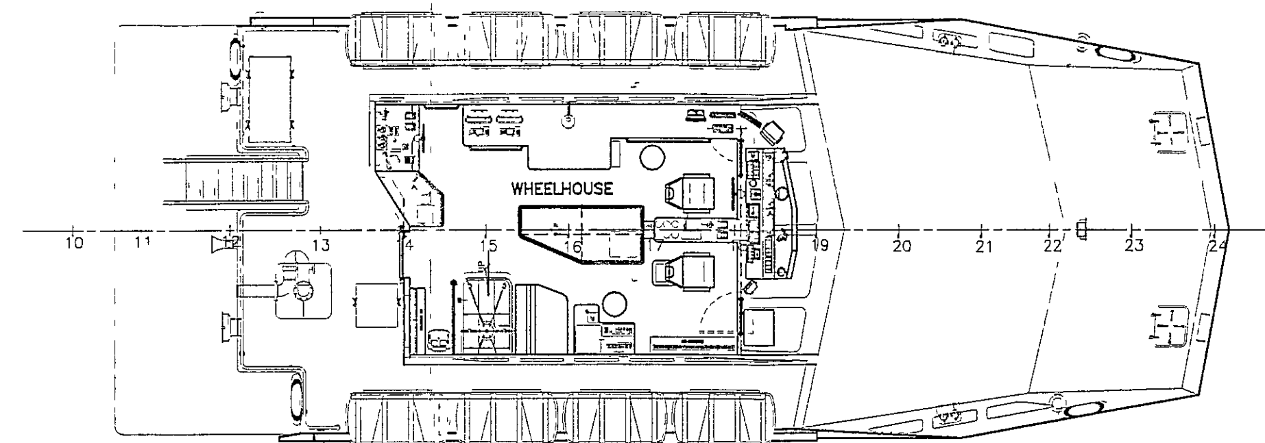
DECKHOUSE PLAN SCALE 1:75
