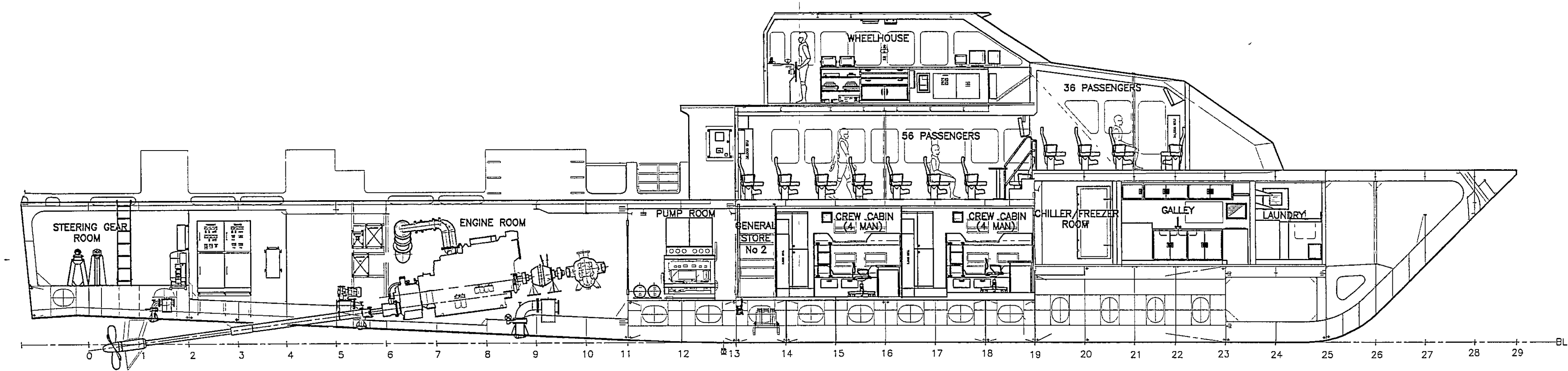
PROFILE SCALE 1:75
