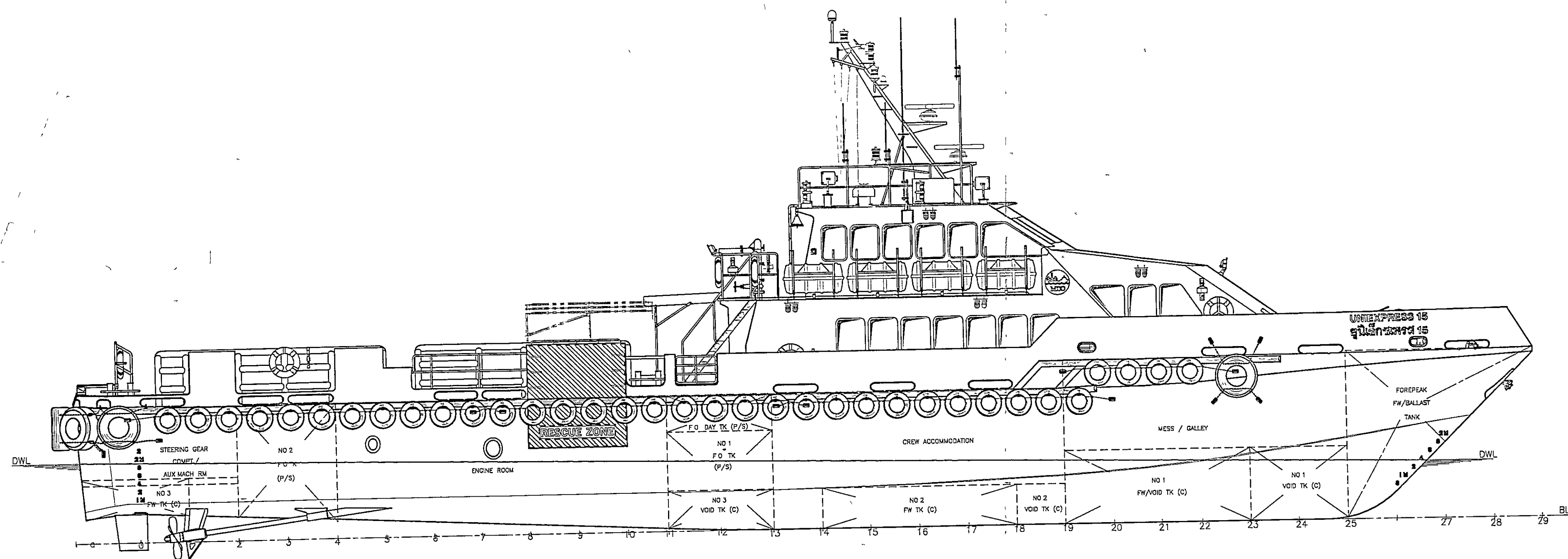
PROFILE SCALE 1/75
