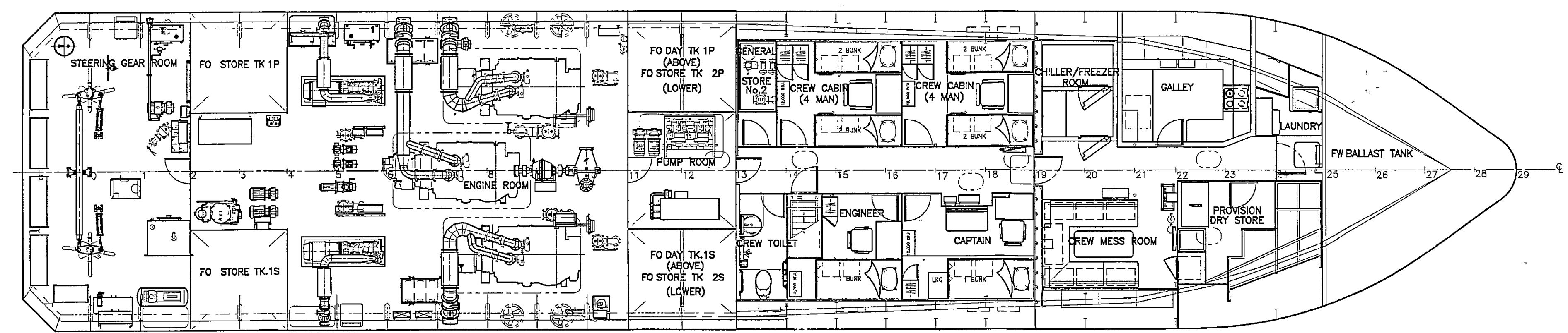
BELOW MAIN DECK SCALE 1:75
