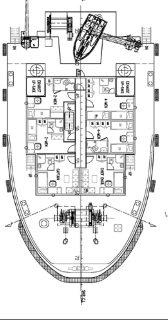
FORECASTLE DECK
