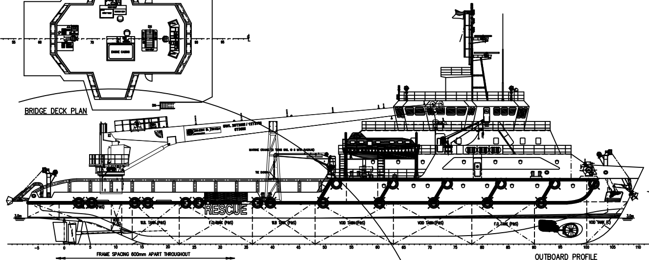
OUTBOARD PROFILE
