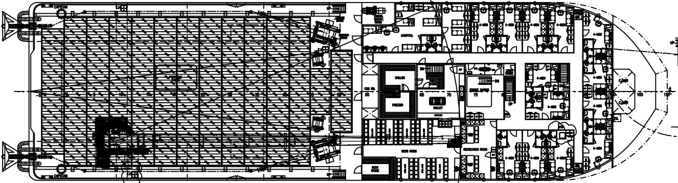
MAIN DECK PLAN 14 x 4 MEN = 56 MEN TOTAL = 56 MEN
