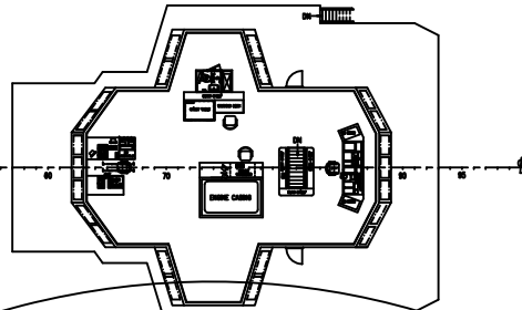
BRIDGE DECK PLAN
