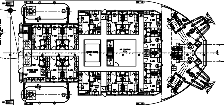
FORECASTLE DECK PLAN 2 x 2 MEN = 4 MEN 13 x 4 MEN = 52 MEN TOTAL = 56 MEN
