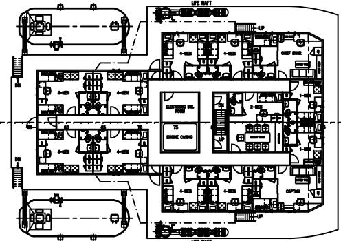
OFFICERS DECK PLAN 4 x 1 MAN = 4 MEN 1 x 2 MEN = 2 MEN 8 x 4 MEN = 32 MEN TOTAL = 38 MEN
