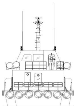
STERN VIEW
