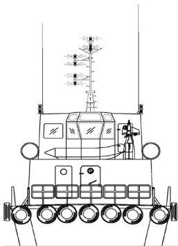
STERN VIEW
