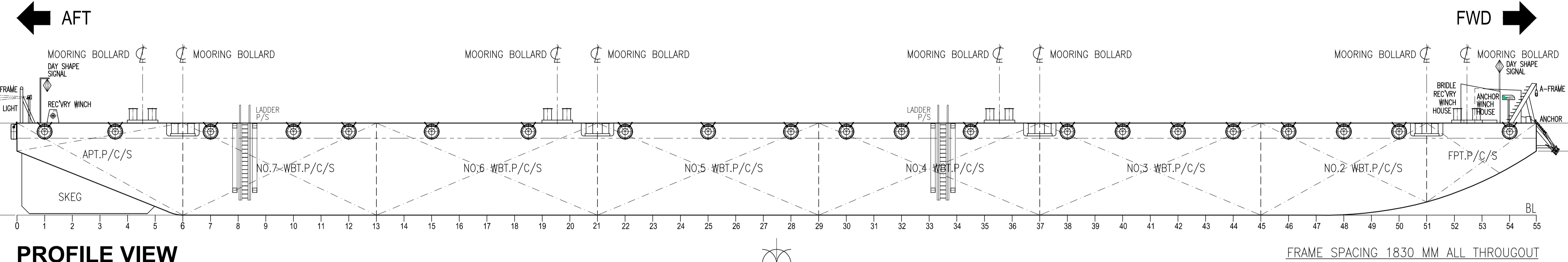
PROFILE VIEW SCALE/ N.T.S (STBD SHOWN)
