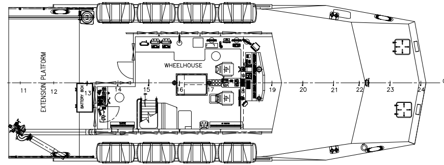
DECKHOUSE PLAN SCALE 1:75
