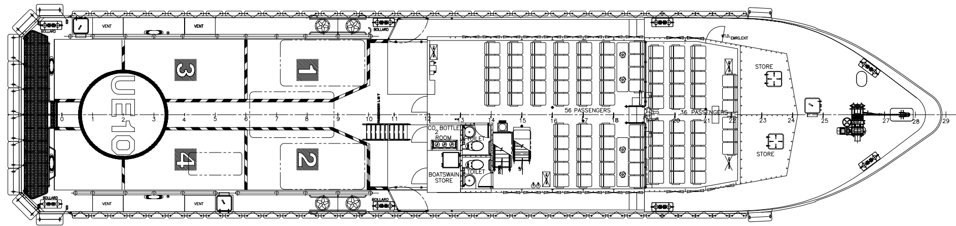
MAIN DECK SCALE 1:75
