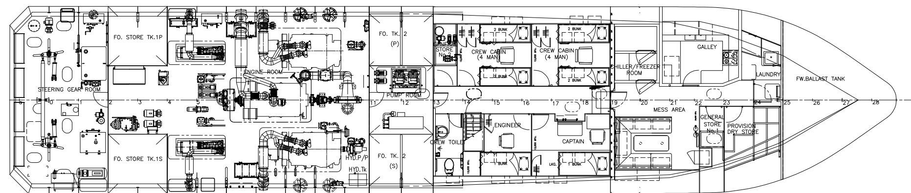
BELOW MAIN DECK SCALE 1:75
