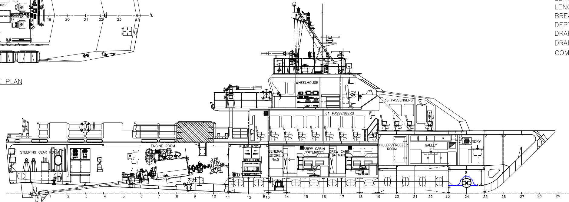
PROFILE SCALE 1:75
