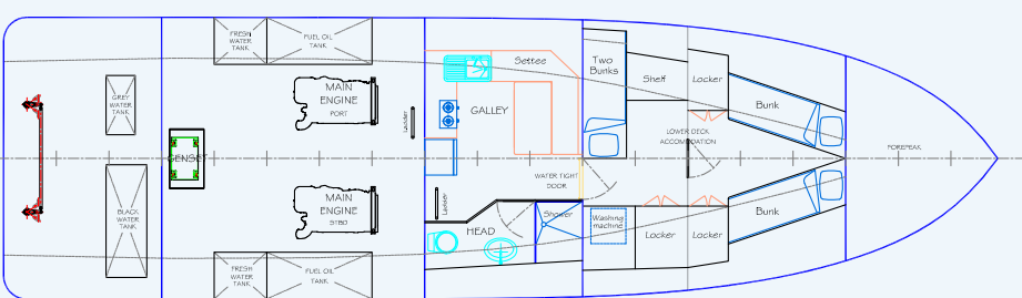
Below Deck Arrangement
