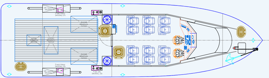
Main Deck Arrangement
